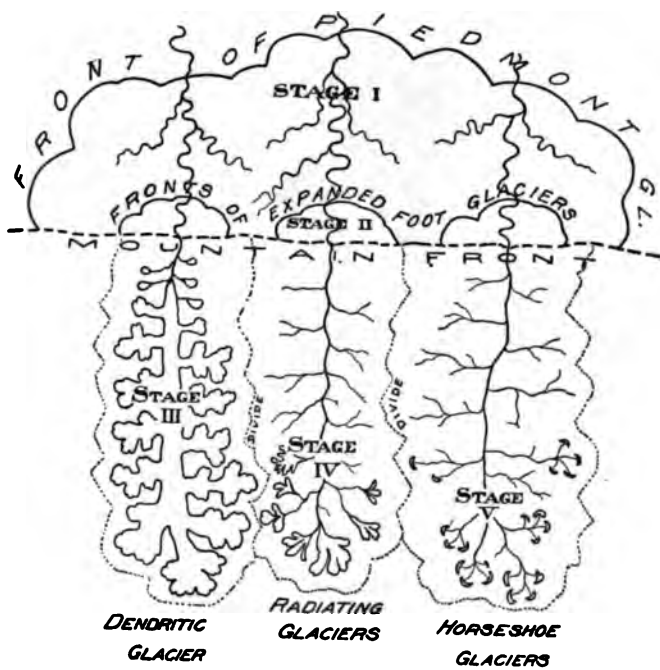
3. 408. — Schematic diagram to show the relationships of glacier types formed in succession during a receding hemicycle of glaciation.
